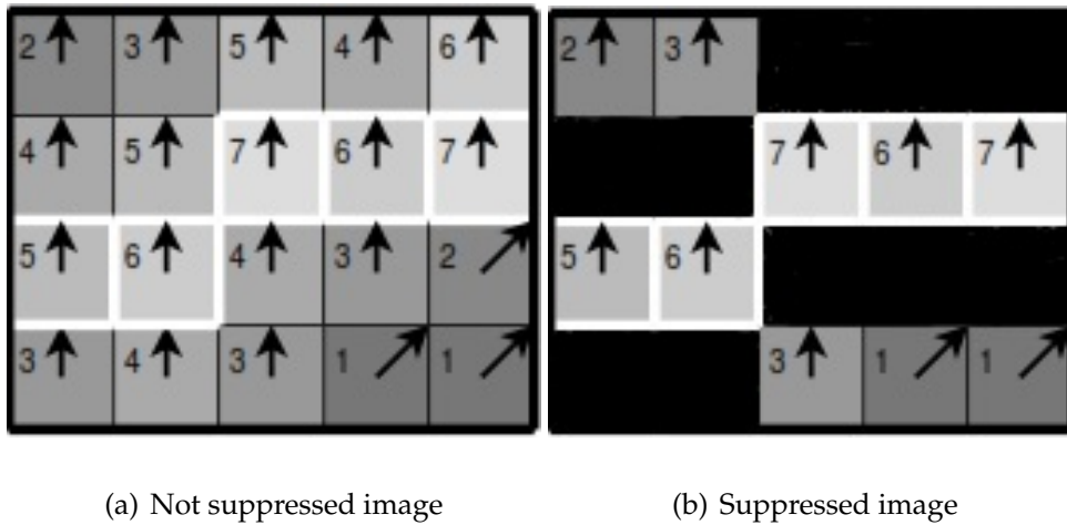
Figure 3.3: Example of non-maximum suppression. The edge strengths are indicated both as colors and numbers, while the gradient directions are shown as arrows. The resulting edge pixels are marked with white borders.
