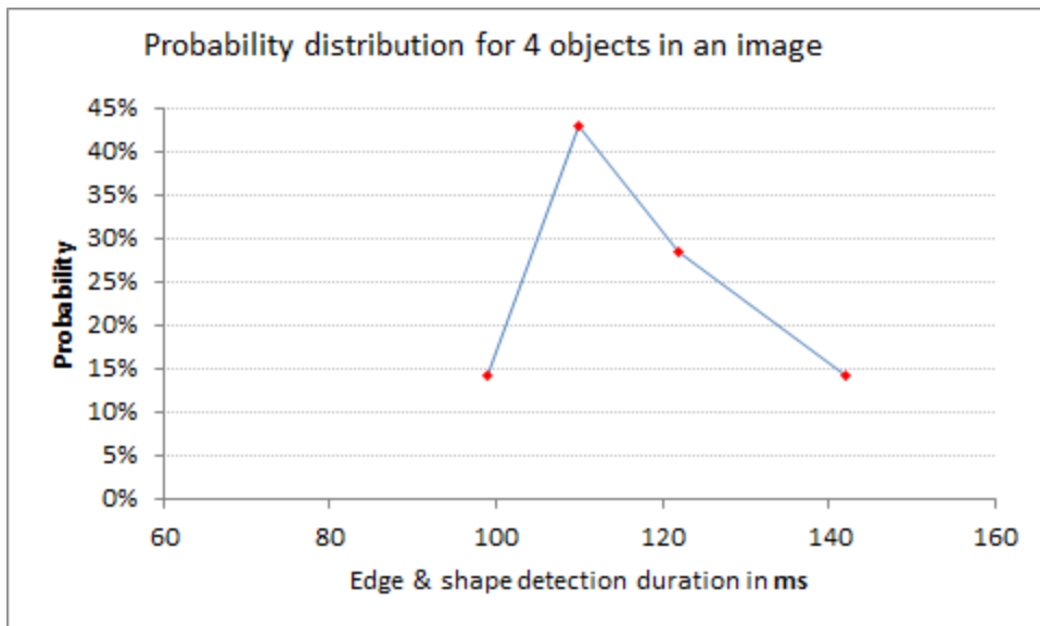
(a) Shape processing time (four objects per image)
