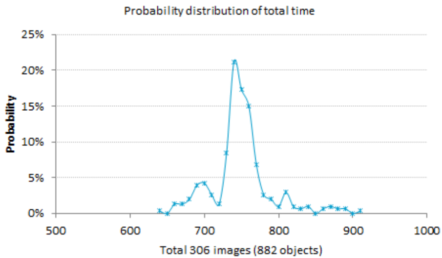
(a) Total Processing Time
