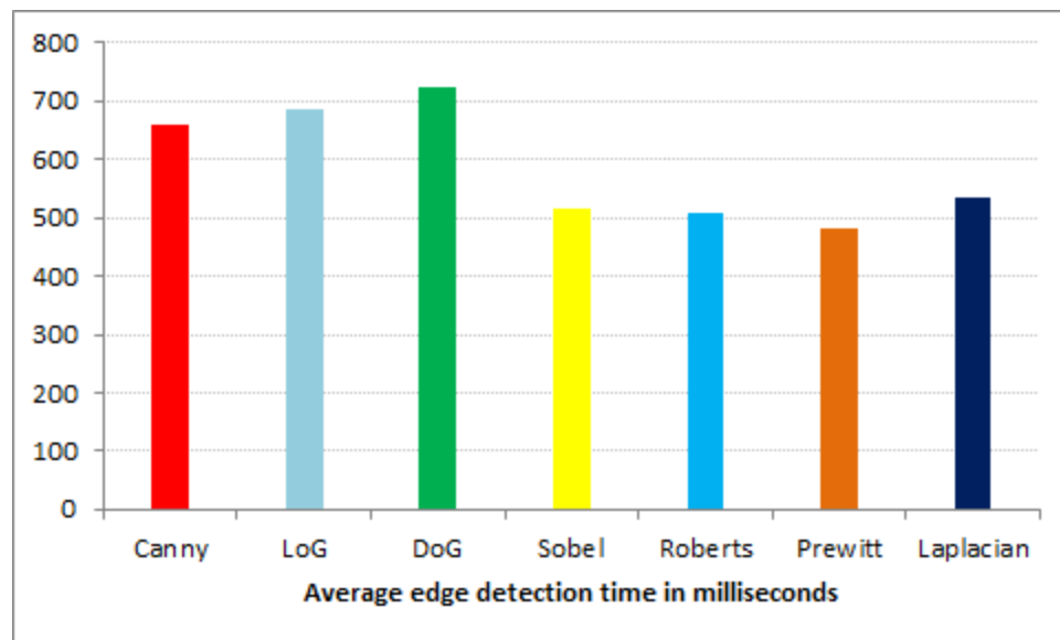
(b) Mean processing time for different techniques
